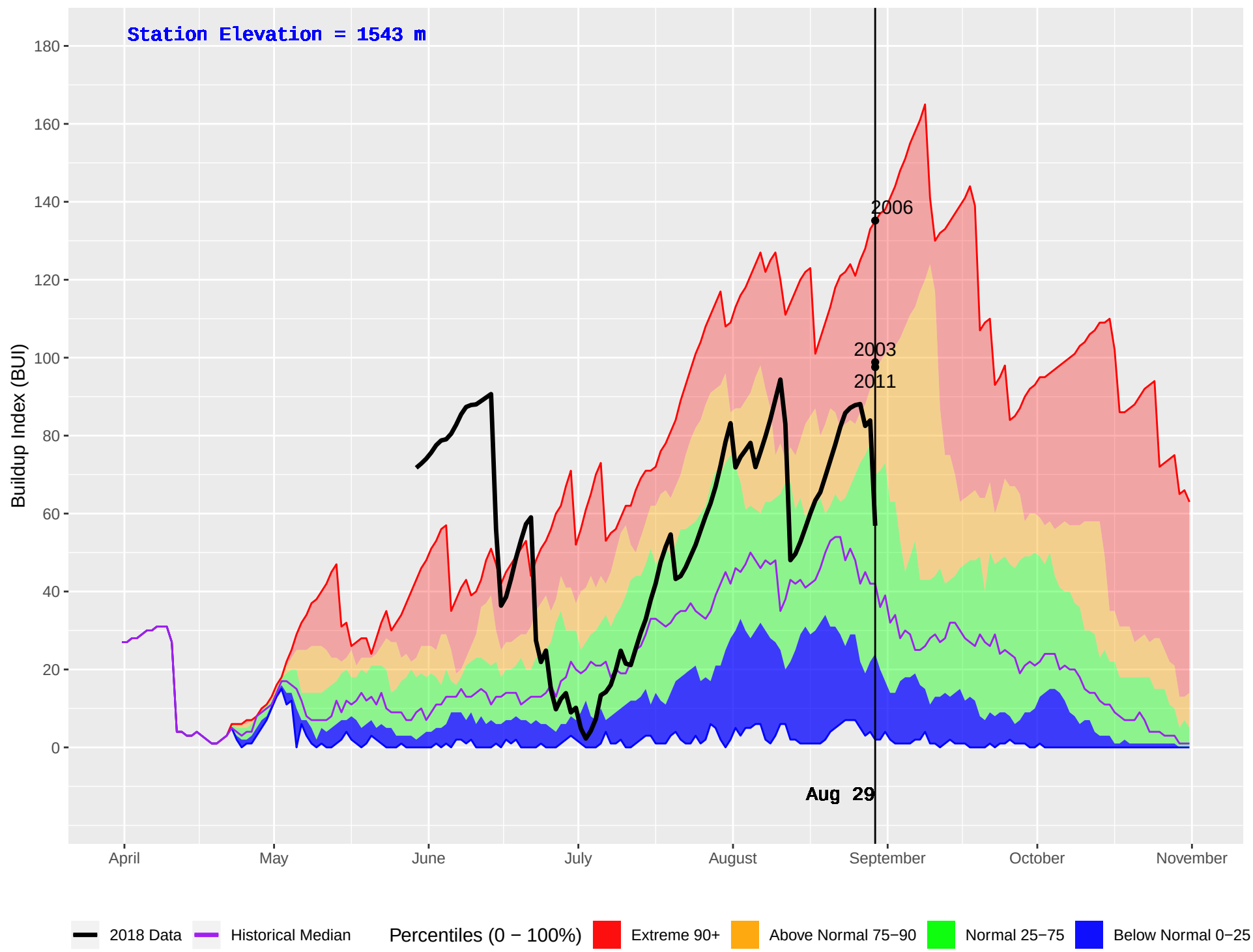
CAHILTY (253) : Historical (1987–2016) and Current (2018) Daily Buildup Index (BUI)
