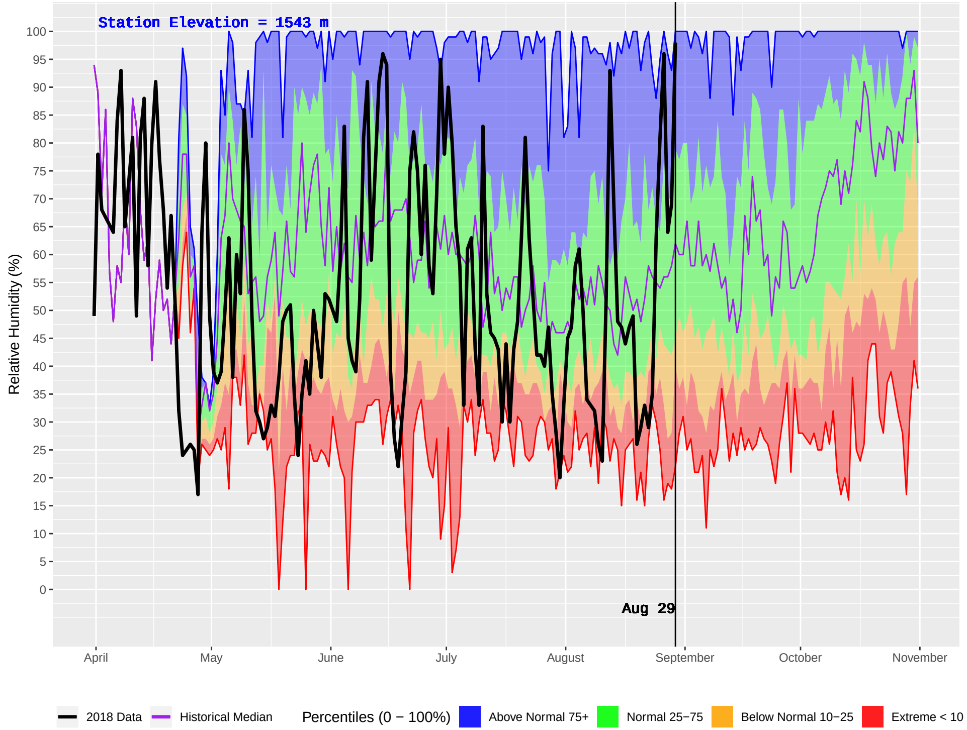
CAHILTY (253) : Historical (1987–2016) and Current (2018) Daily Relative Humidity
