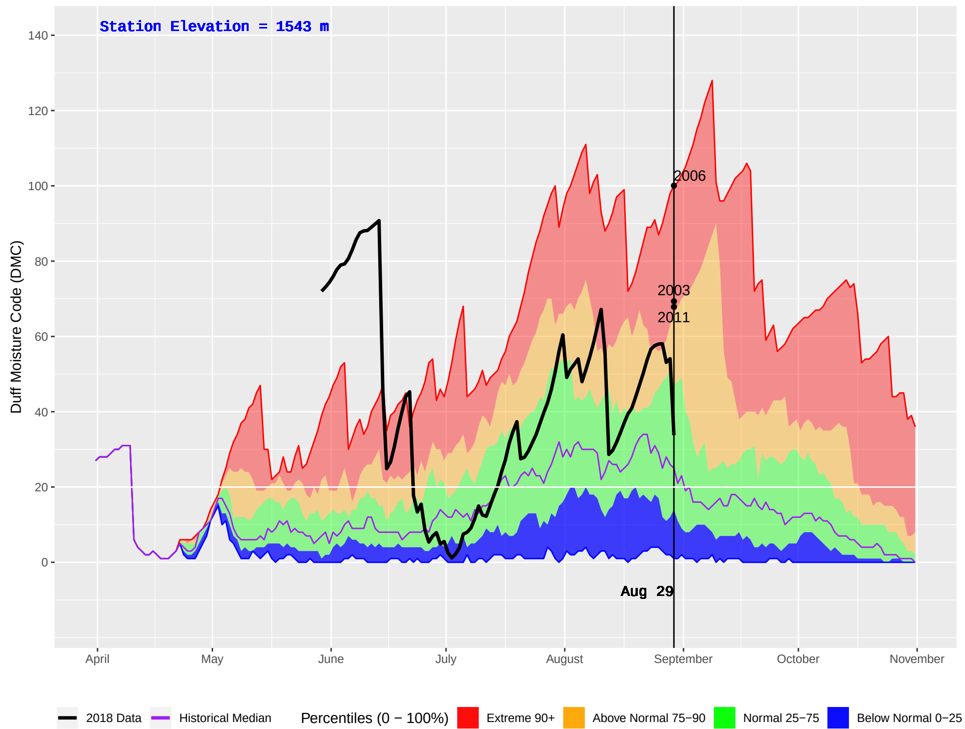
CAHILTY (253) : Historical (1987–2016) and Current (2018) Daily Duff Moisture Code (DMC)
