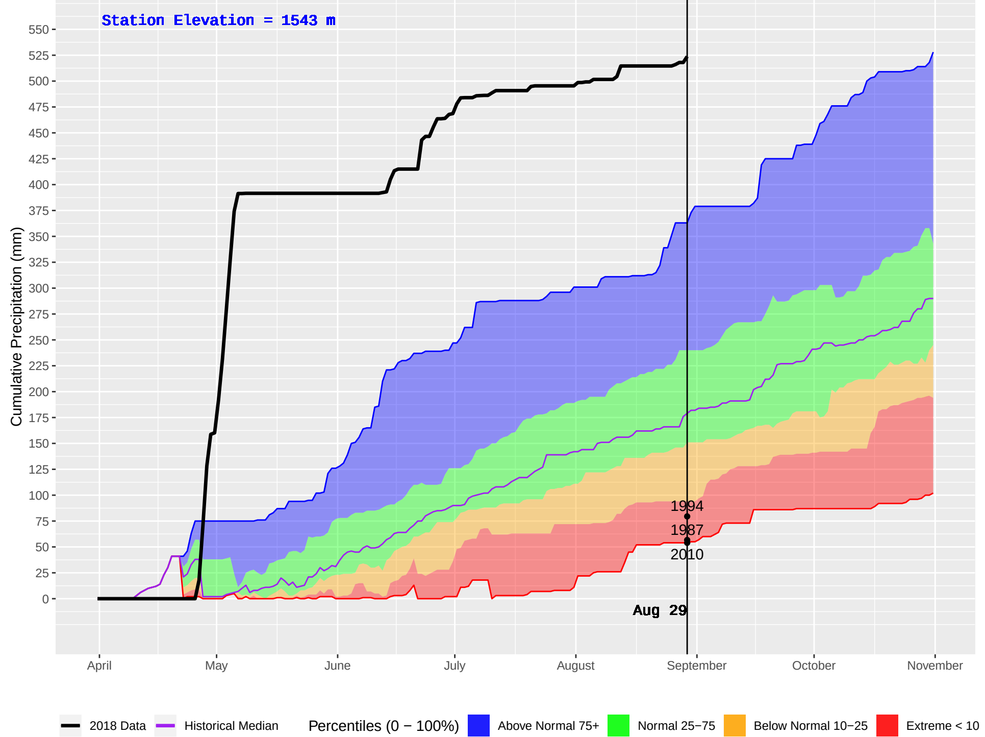
CAHILTY (253) : Historical (1987–2016) and Current (2018) Daily Cumulative Precipitation
