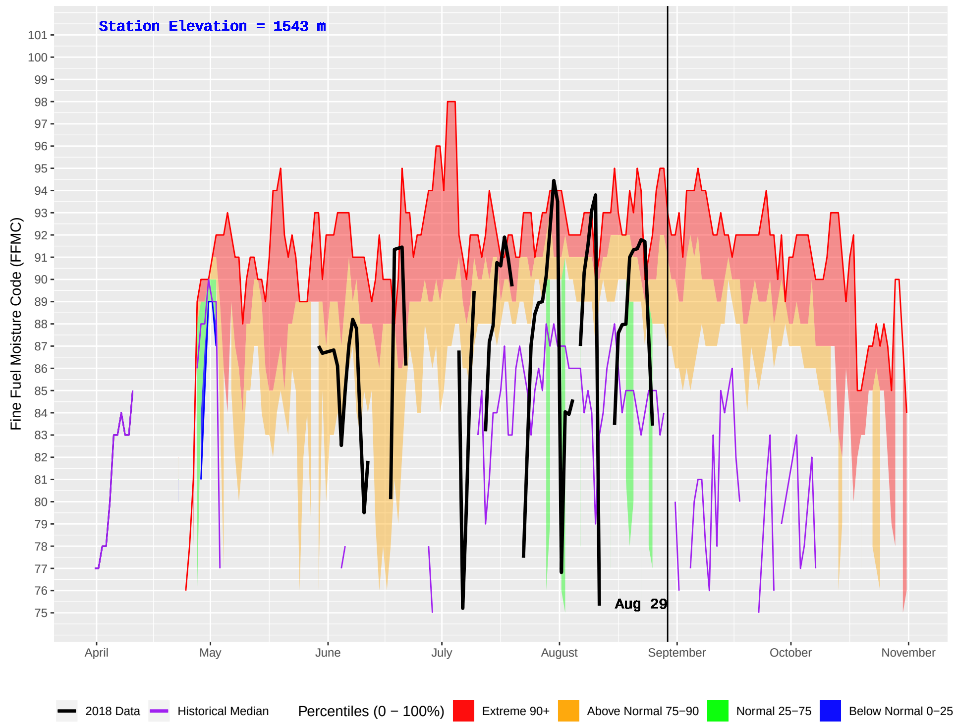
CAHILTY (253) : Historical (1987–2016) and Current (2018) Daily Fine Fuel Moisture Code (FFMC)
