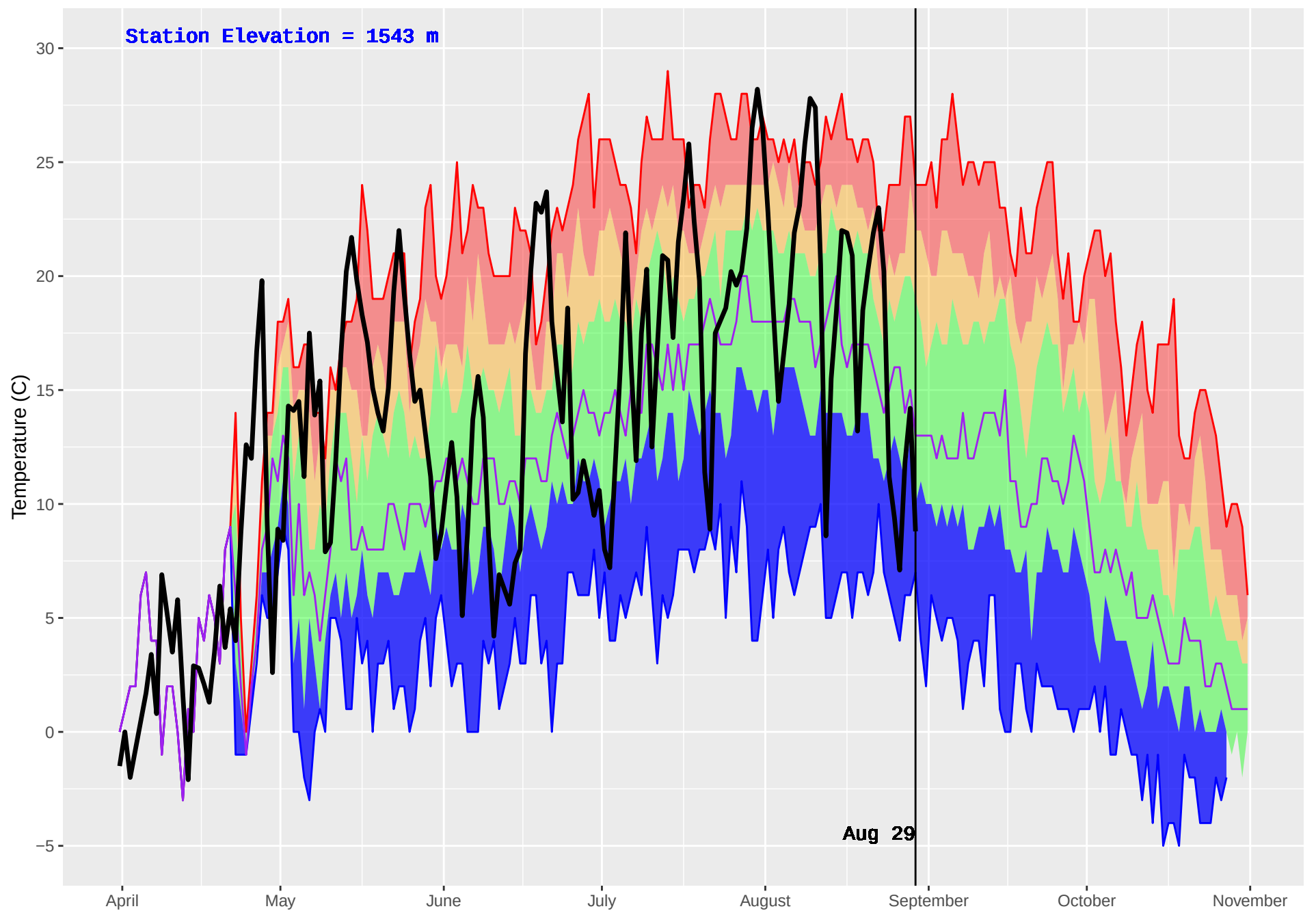
CAHILTY (253) : Historical (1987–2016) and Current (2018) Daily Temperature
