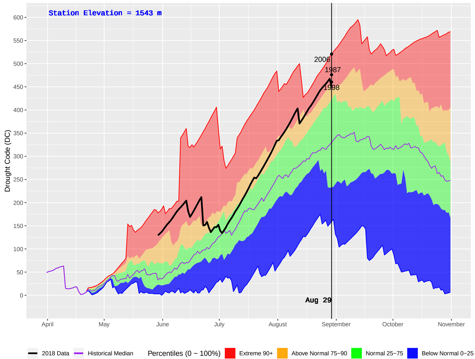
CAHILTY (253) : Historical (1987–2016) and Current (2018) Daily Drought Code (DC)
